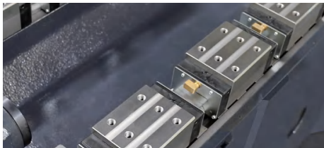
X/Z axis roller linear guideway with 3 sliders
