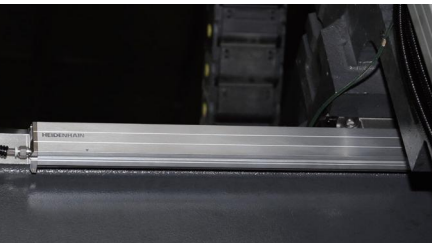
Fully closed-loop linear scale (X/Y/Z/A/C axis)
