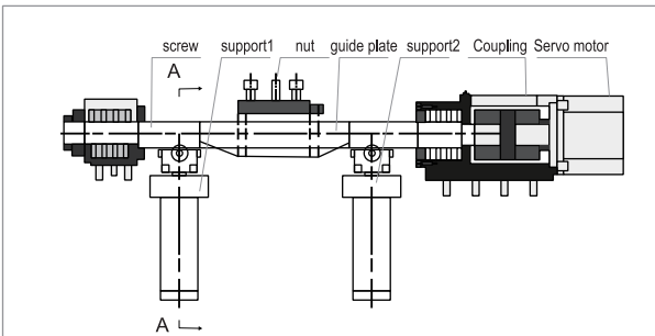
Ball screw support structure
