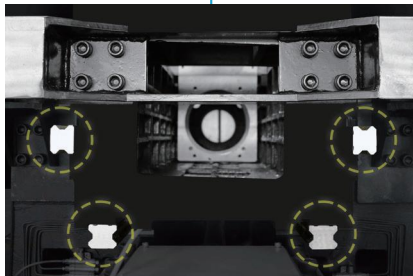
Z axis 4 linear guideway Z-axis 4-linear guideway is located in four directions and receives force at equal intervals, effectively improving cutting capabilities.
