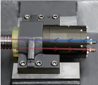
Hollow oil-cooled ball screw
