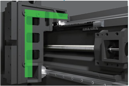
BAOFENG inverted L-shaped Y-axis design Y-axis adopts a long-span inverted L-shaped design, and the center of gravity falls on the column, which reduces the cantilever length of ram spindle and effectively improves the rigidity of Y-axis and cutting rigidity of the head.
