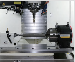
4th axis rotary table
