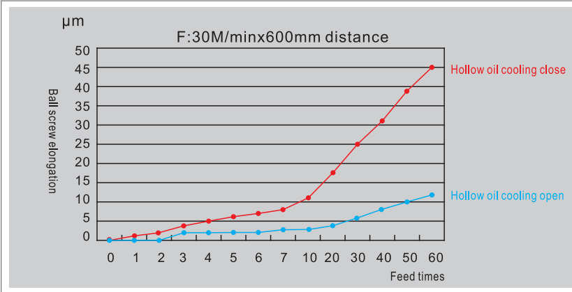
Comparison table of positioning accuracy with ball screw cooling device and without ball screw cooling device
