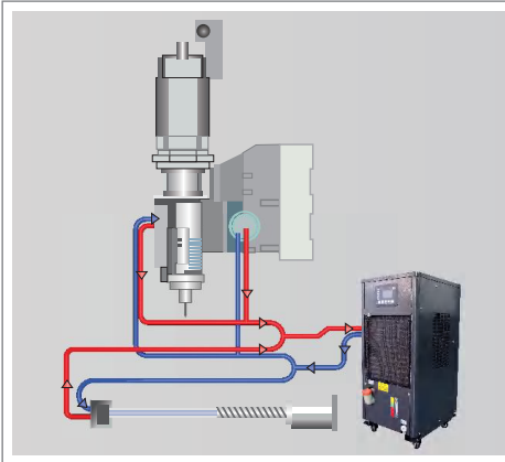
Spindle and 3 axis ball screw cooling device
